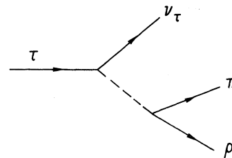
FIG. 1. Diagram for \tau decay.
